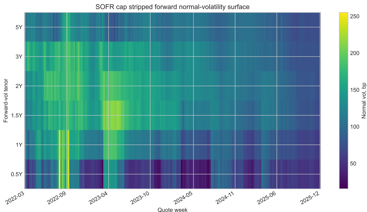
Figure 1: Stripped SOFR forward normal-volatility surface. Each date carries a full forward-tenor curve, so the figure shows both cross-sectional term structure and time-series evolution.
