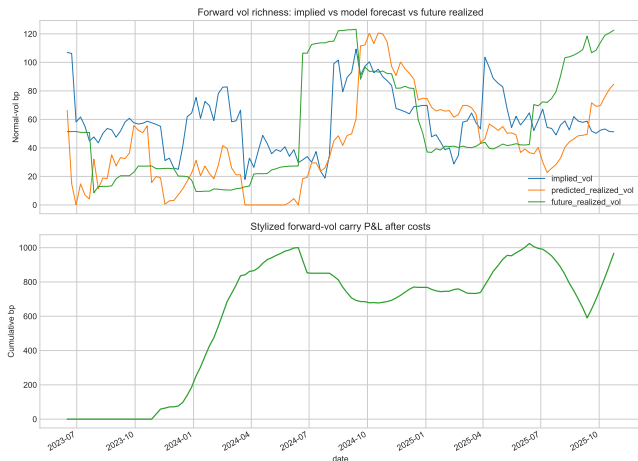
Figure 8: Walk-forward implied vol, predicted realized vol, future realized vol, and cumulative carry proxy P&L.
