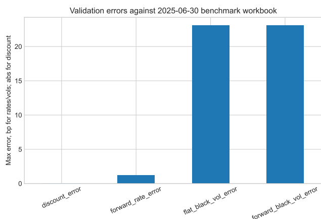
Figure 2: Independent workbook validation of discount factors, forwards, flat Black vols, and stripped forward Black vols.
