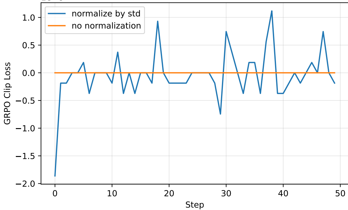
GRPO Training: Loss
