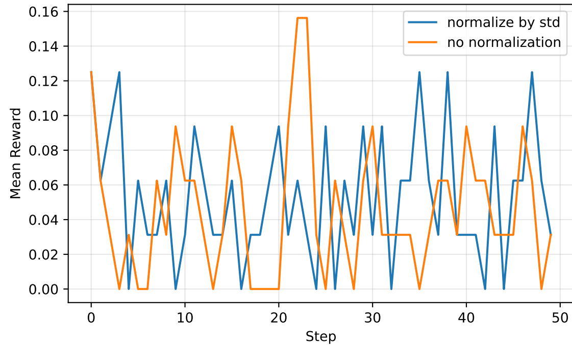
GRPO Training: Mean Reward
