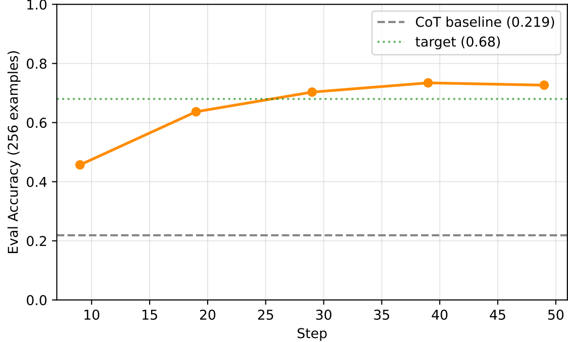
GRPO Validation Accuracy
