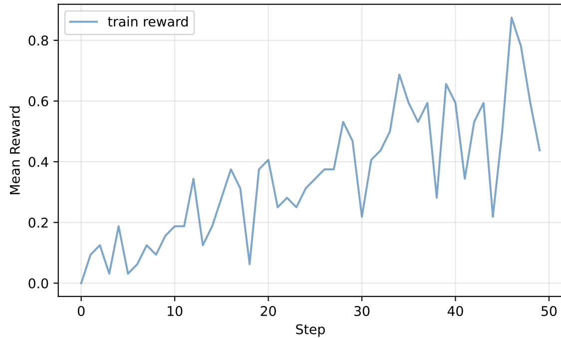
GRPO Training: Rollout Reward
