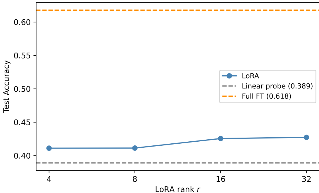
LoRA Rank Sweep on RESISC45
