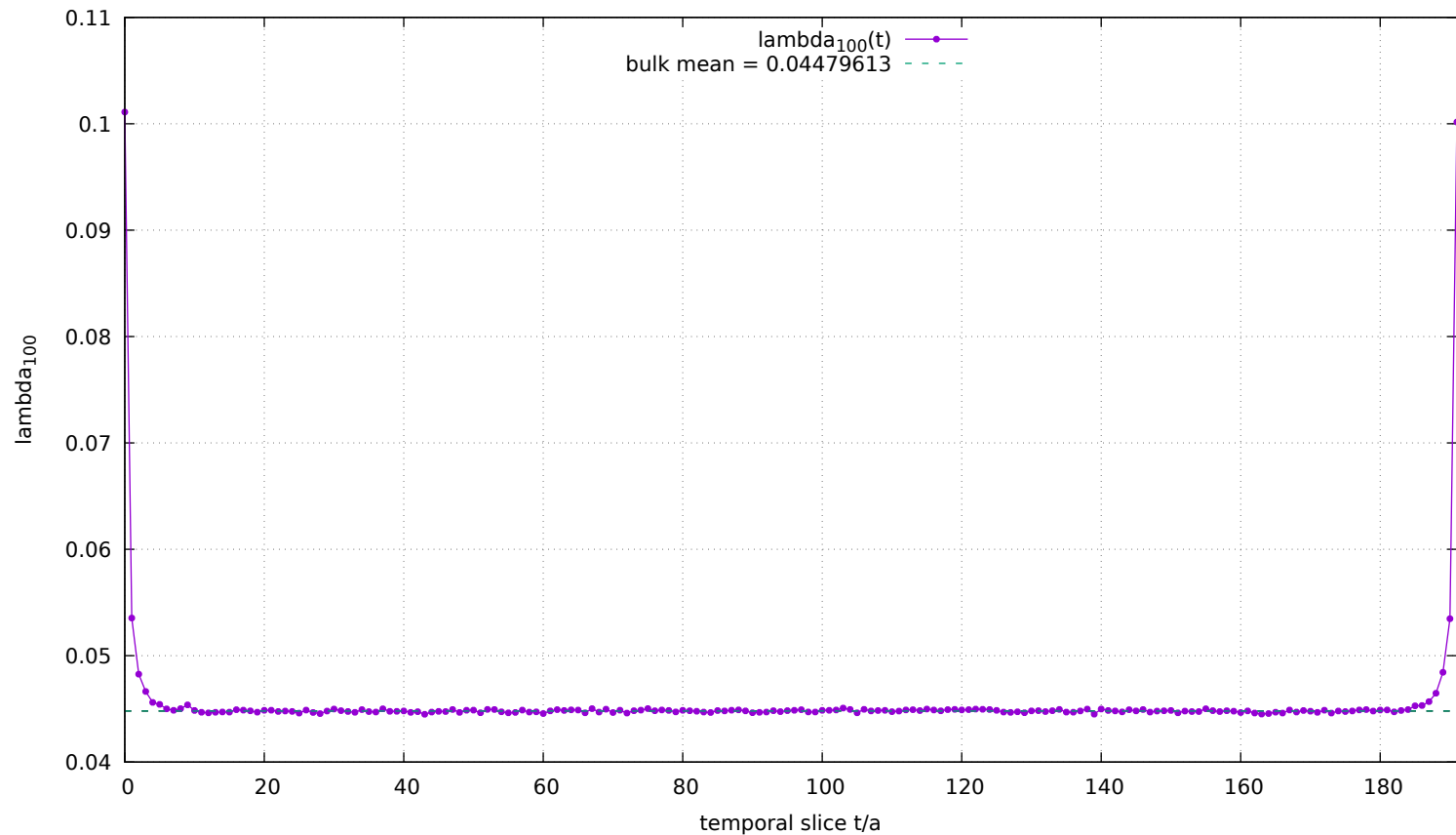
qX p2n100: 100th covariant-Laplacian eigenvalue
