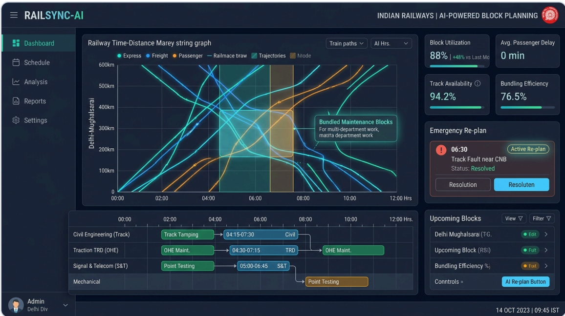
RAILSYNC-AI Dashboard Cockpit
