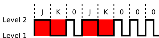
Starting delimiter of Token Ring
