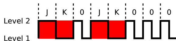
Starting delimiter of Token Ring
