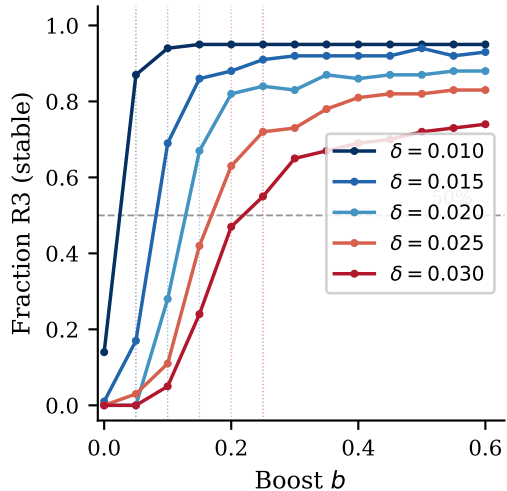
(a) Bifurcation by degradation rate
