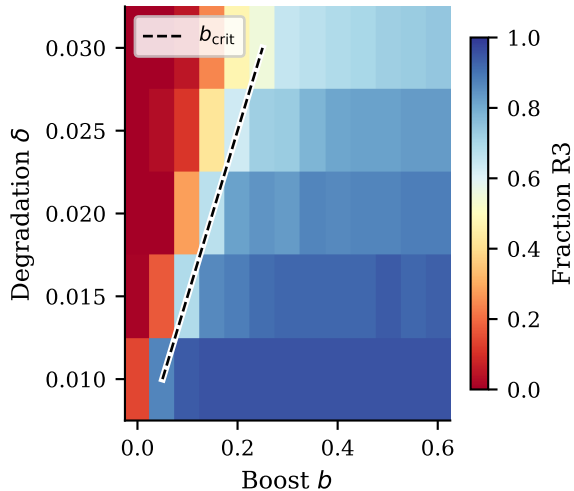
(b) Regime phase diagram
