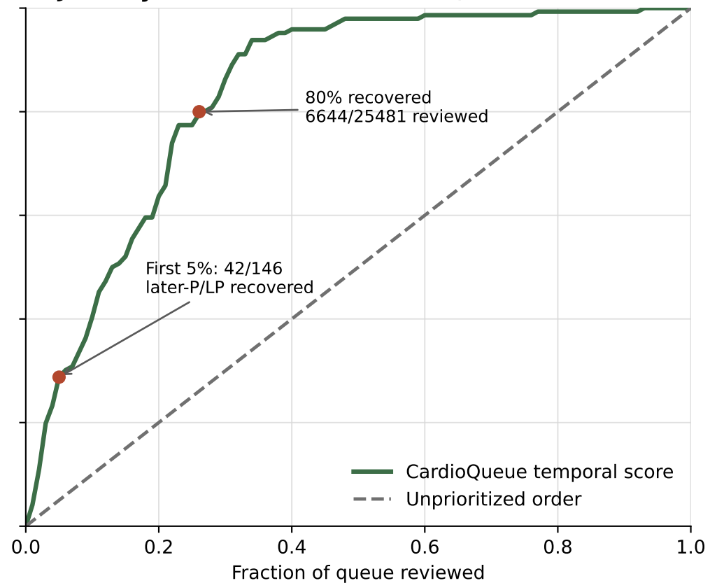
B January 2024 VUS cohort (n=25,481)
