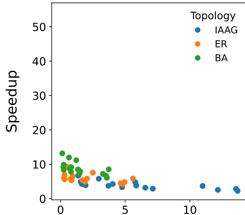
Flow factor = 1.0
