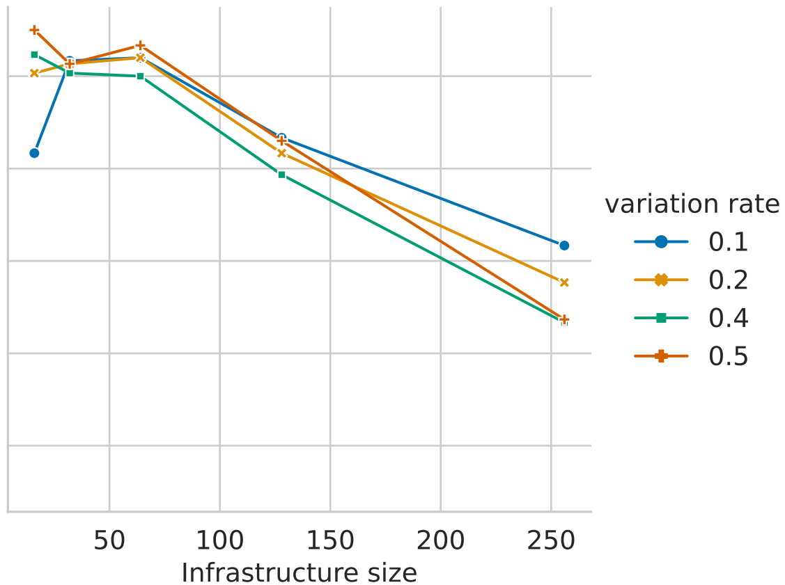
relaxed = True
