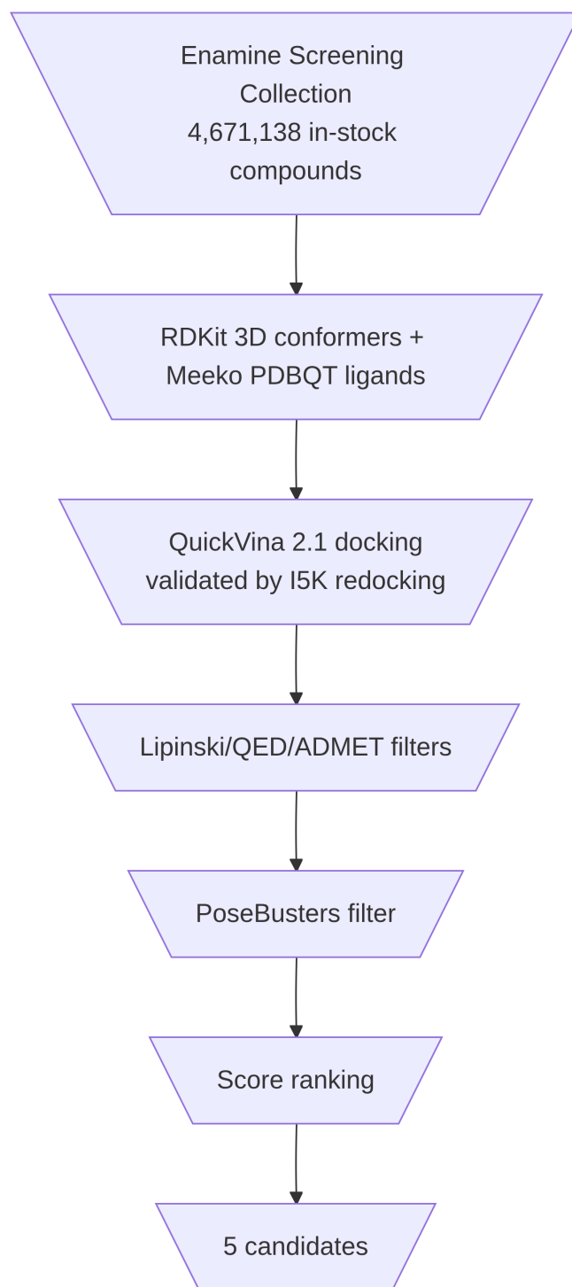
Figure S2: Funnel-shaped virtual-screening pipeline used to prioritize five PfBDP1 candidate ligands from the Enamine Screening Collection.
