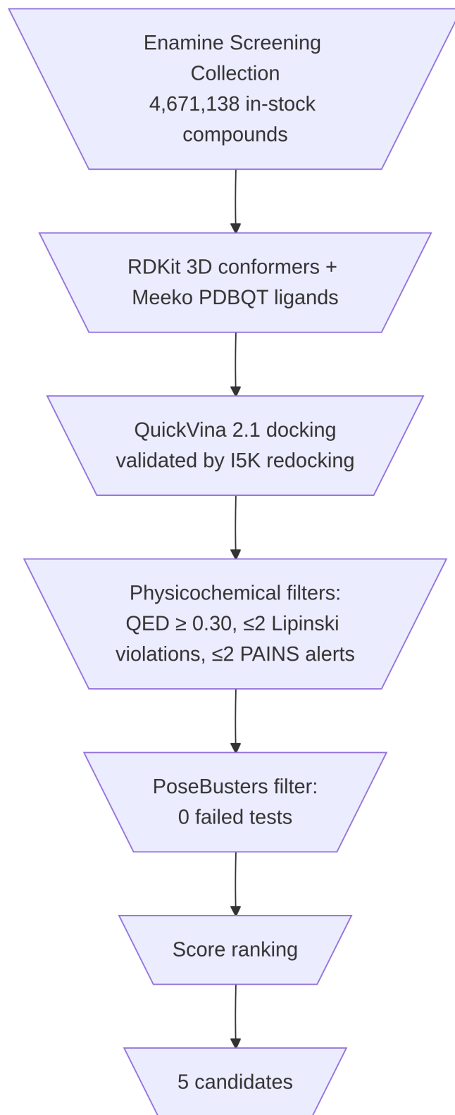
Figure S2: Funnel-shaped virtual-screening pipeline used to prioritize five PfBDP1 candidate ligands from the Enamine Screening Collection. Explicit thresholds ensure reproducibility: minimum QED 0.30, maximum two Lipinski rule-of-five violations, maximum two PAINS alerts, and zero PoseBusters failures.
