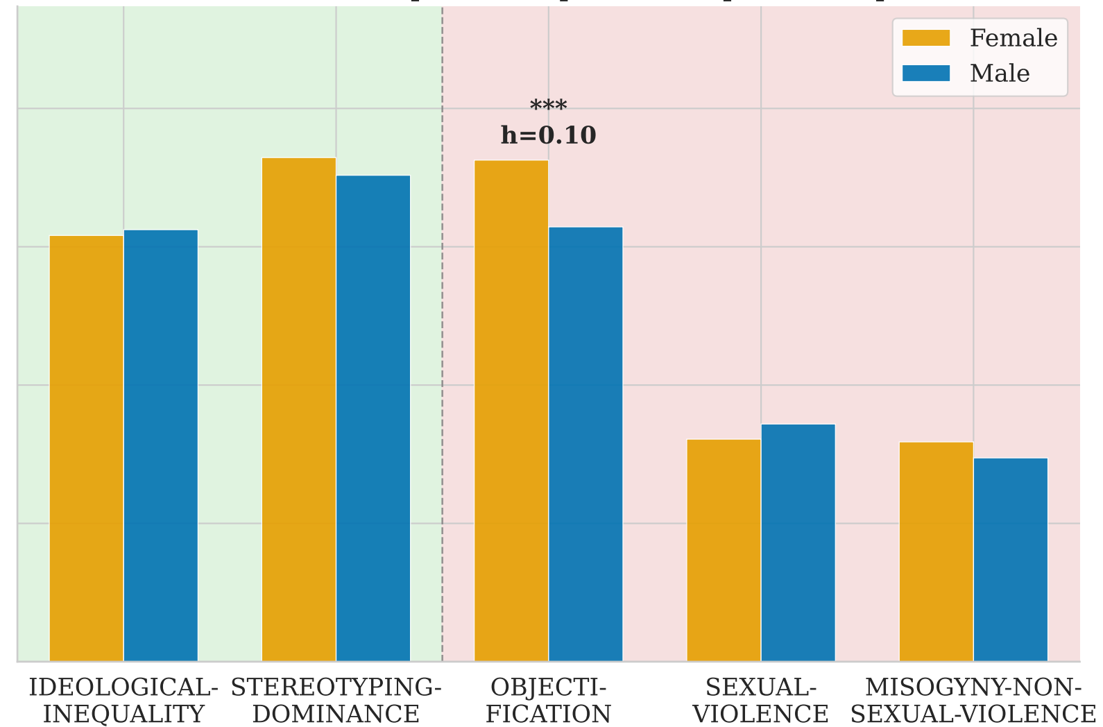
Memes — Gender Shapes Categorisation (Holm-corrected: * p < .05 , ** p < .01 , *** p < .001 , † p < .10 )
