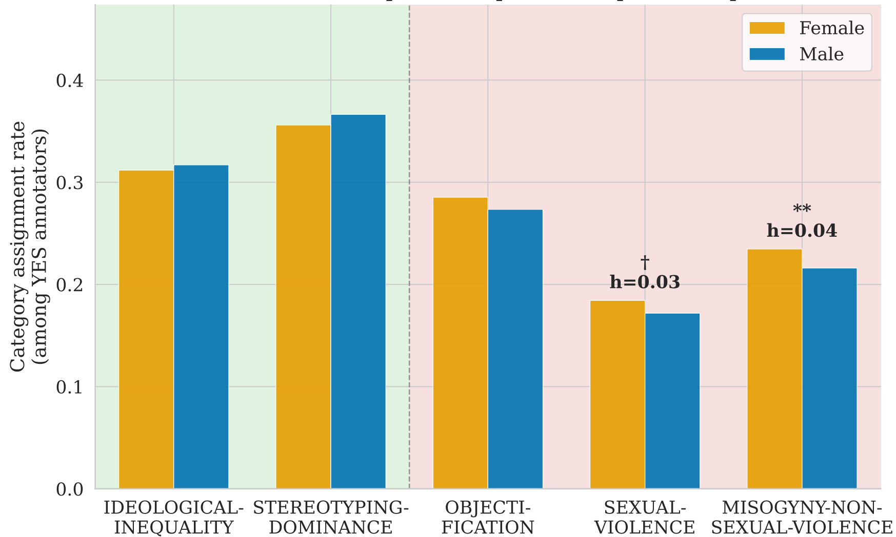
Tweets — Gender Shapes Categorisation (Holm-corrected: * p < .05 , ** p < .01 , *** p < .001 , † p < .10 )
