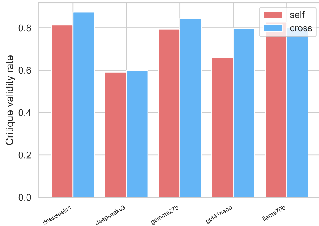
Self vs cross critique validity (per critic)
