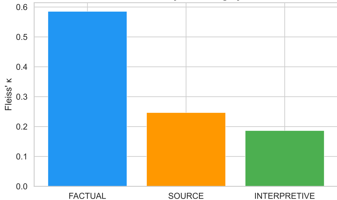
Fleiss' \kappa by CCL Category
