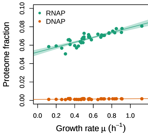
Merged
