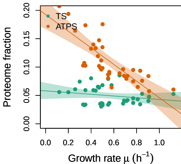
Merged
