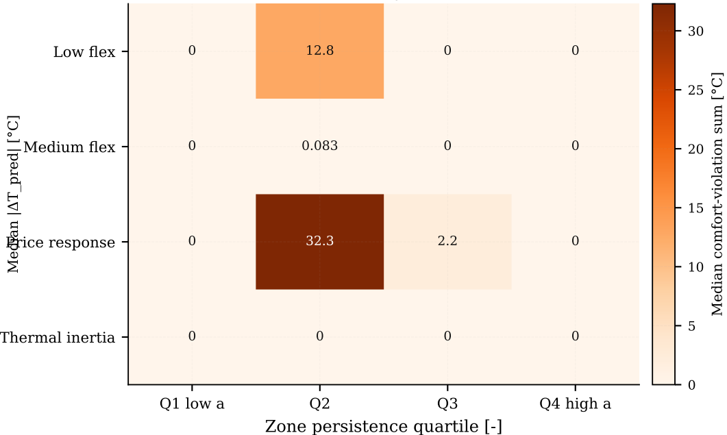
Median comfort-violation sum by inertia class
