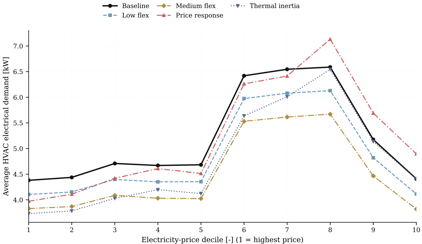
HVAC dispatch by electricity-price class (2022)
