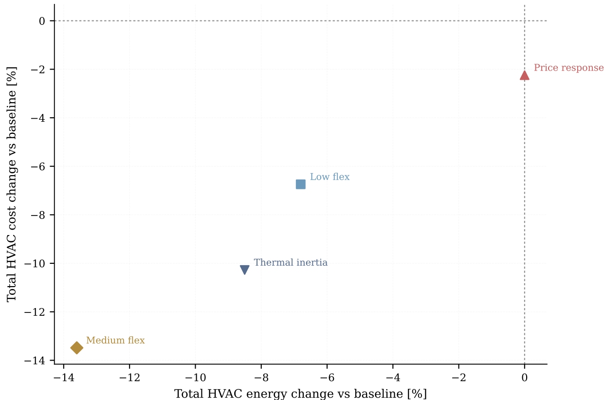
Annual energy-cost-thermal trade-off frontier (2022)
