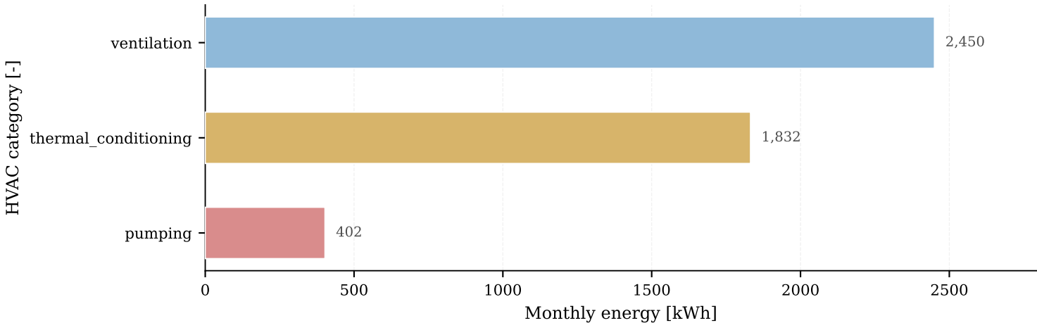
Aggregated HVAC monthly consumption — July
