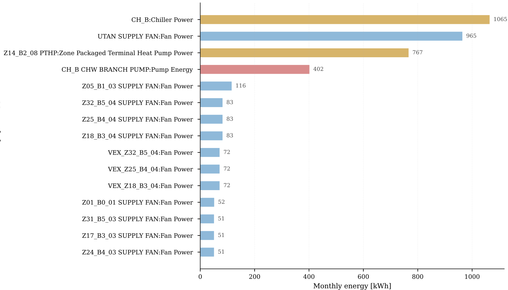
HVAC equipment consumption — top 15 monthly consumers — July
