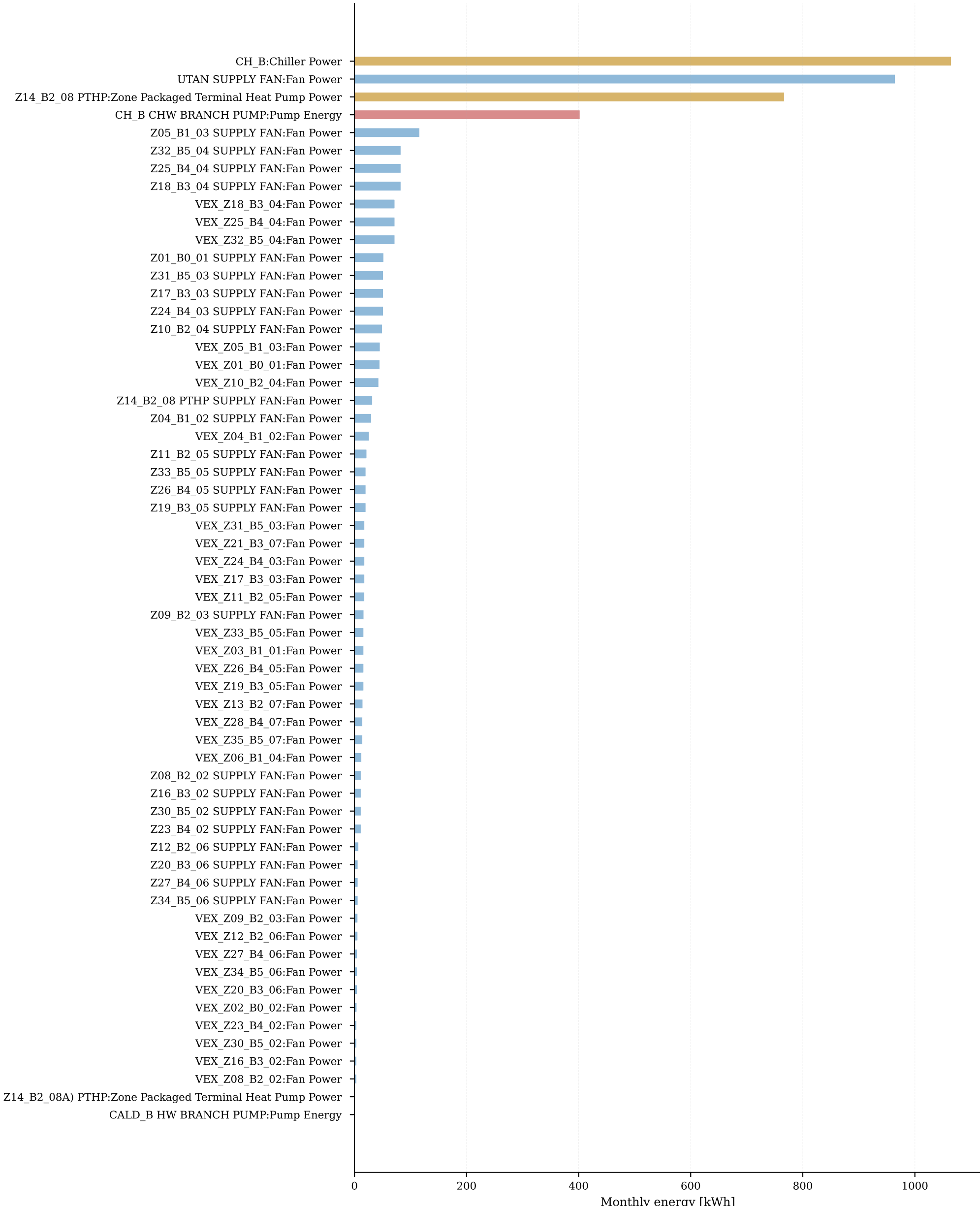
HVAC equipment consumption — ranked monthly profile — July
