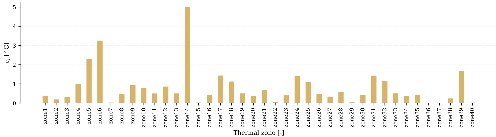
Thermal coefficient c_z by zone
