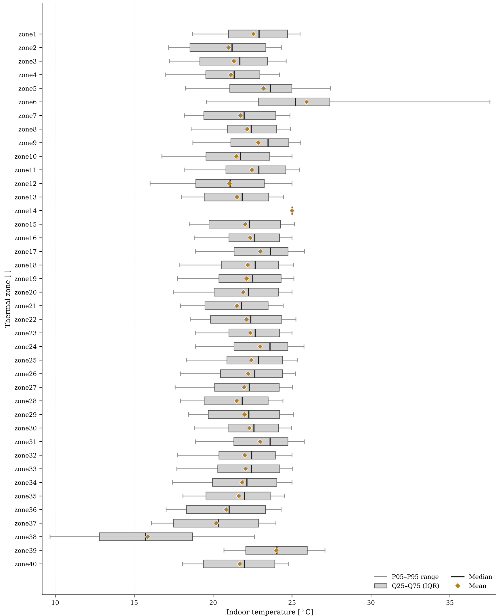
Indoor temperature distribution by thermal zone — 2022
