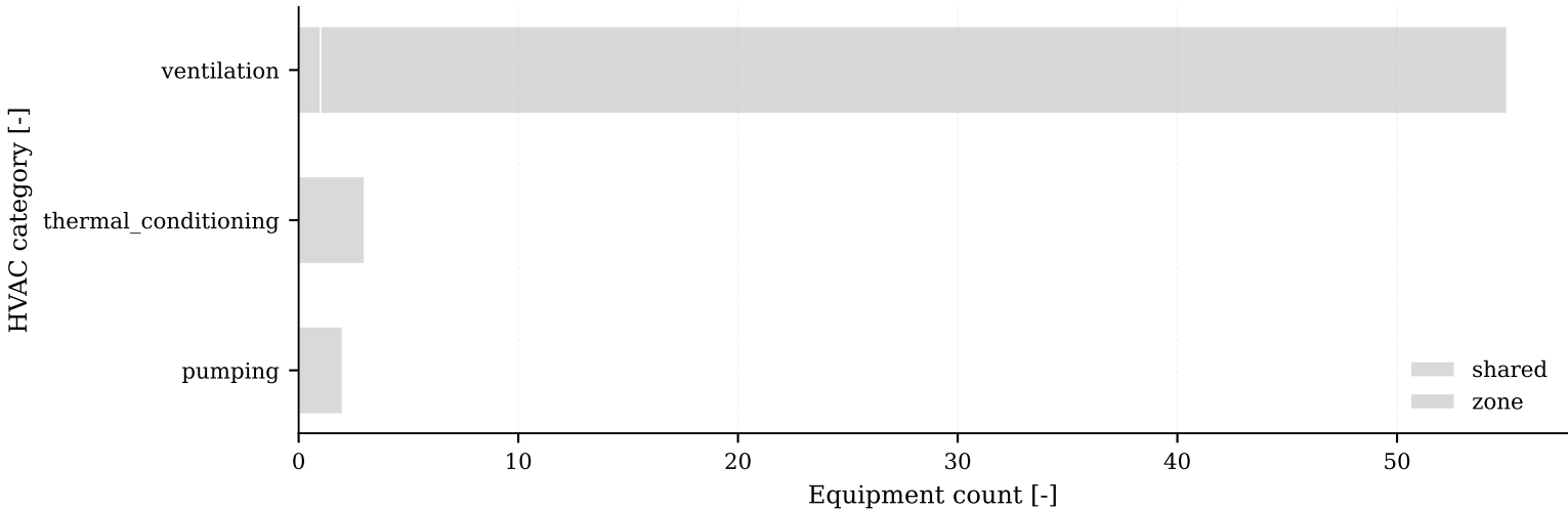
HVAC equipment grouping by service scope
