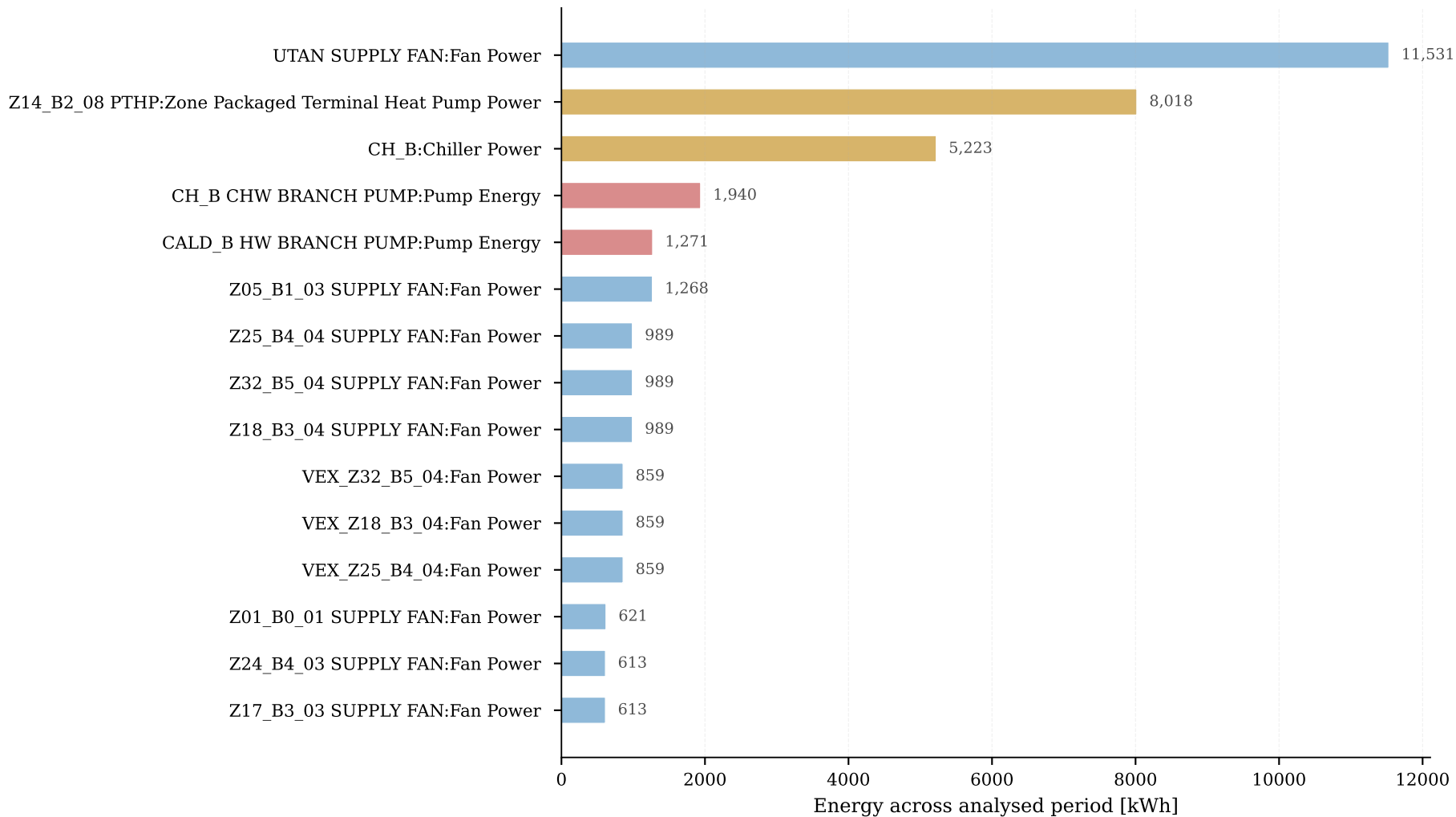
HVAC equipment consumption — top 15 consumers — 2022
