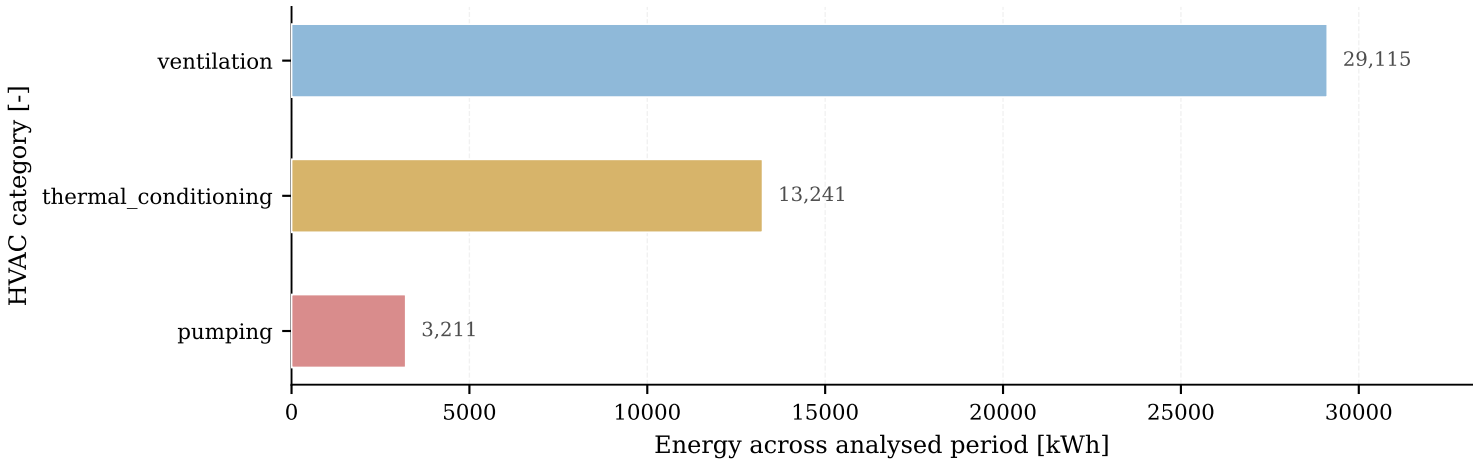
Aggregated HVAC energy consumption by category — 2022
