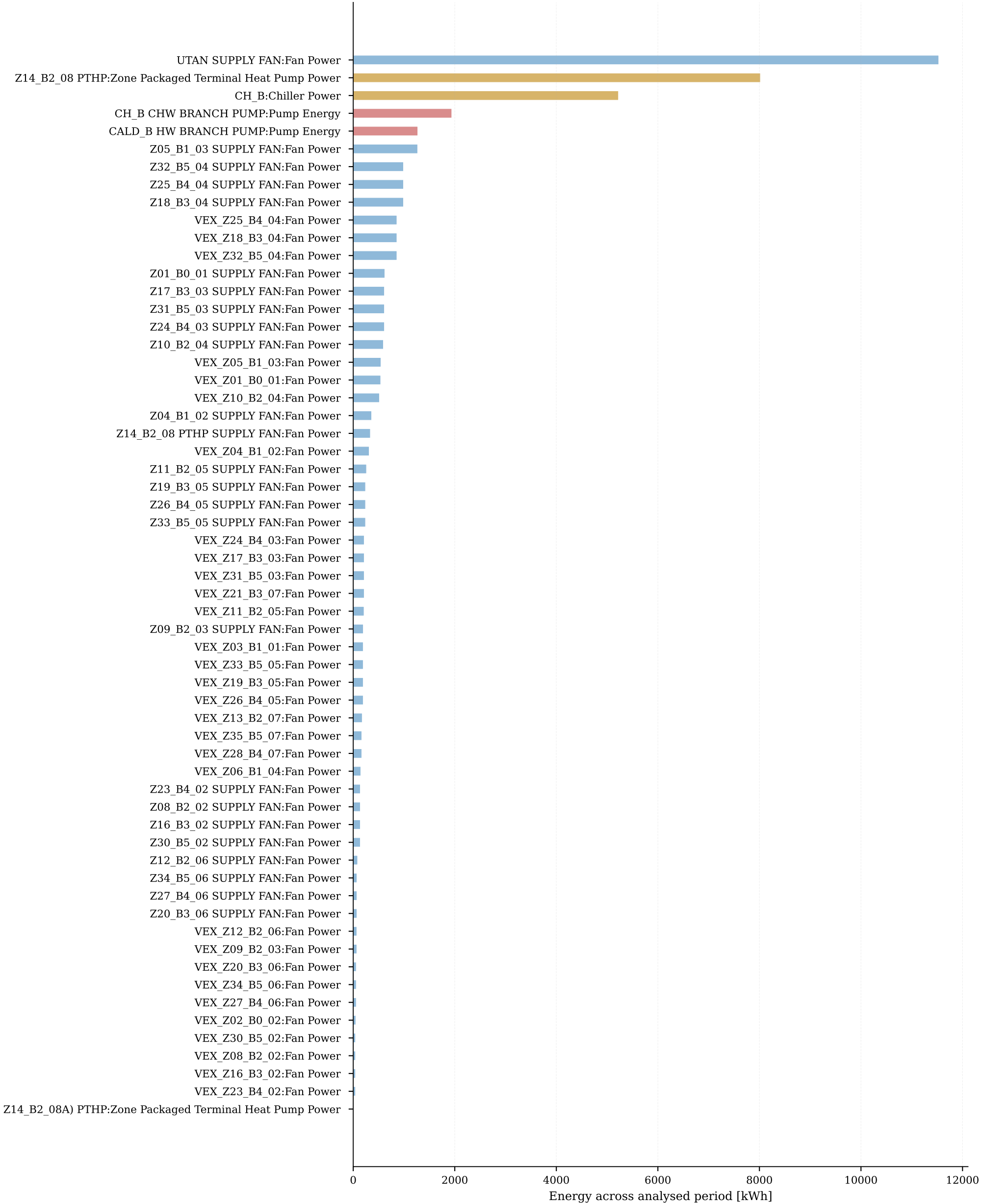
HVAC equipment consumption — ranked profile — 2022
