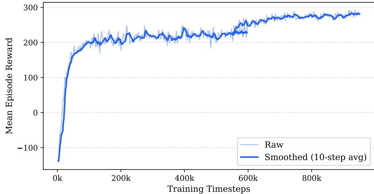
PPO Training Curve
