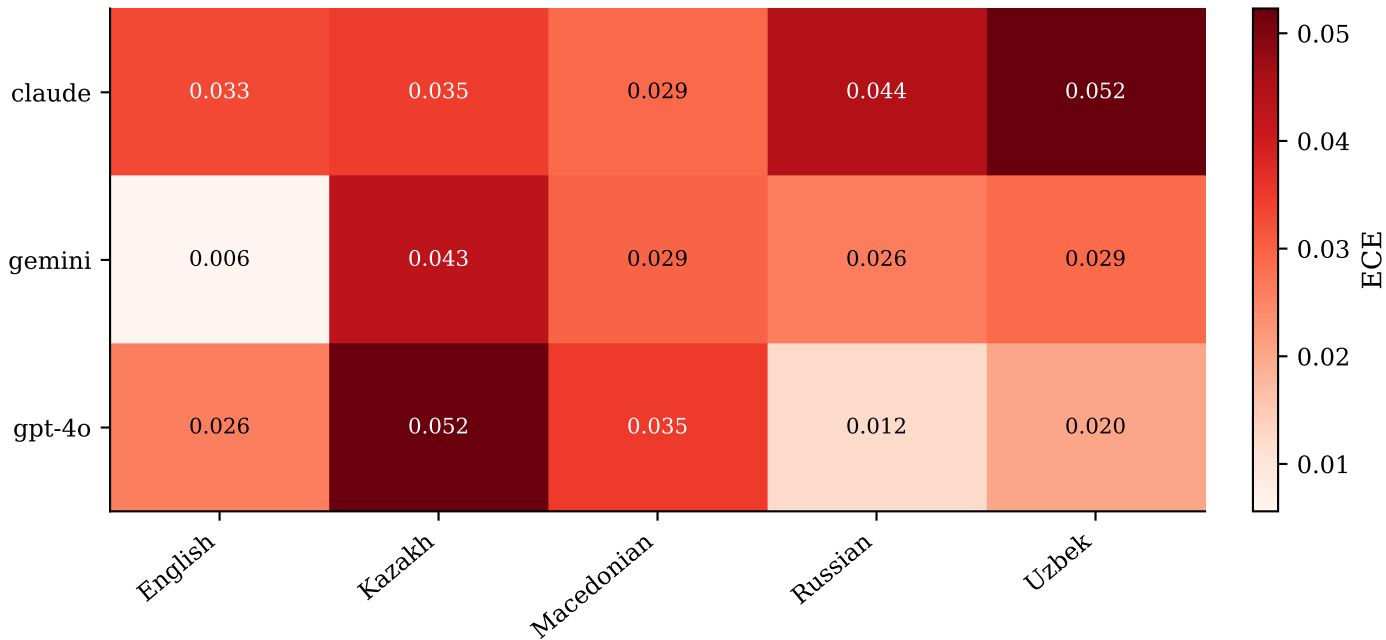
Calibration Error (ECE) by Model and Language
