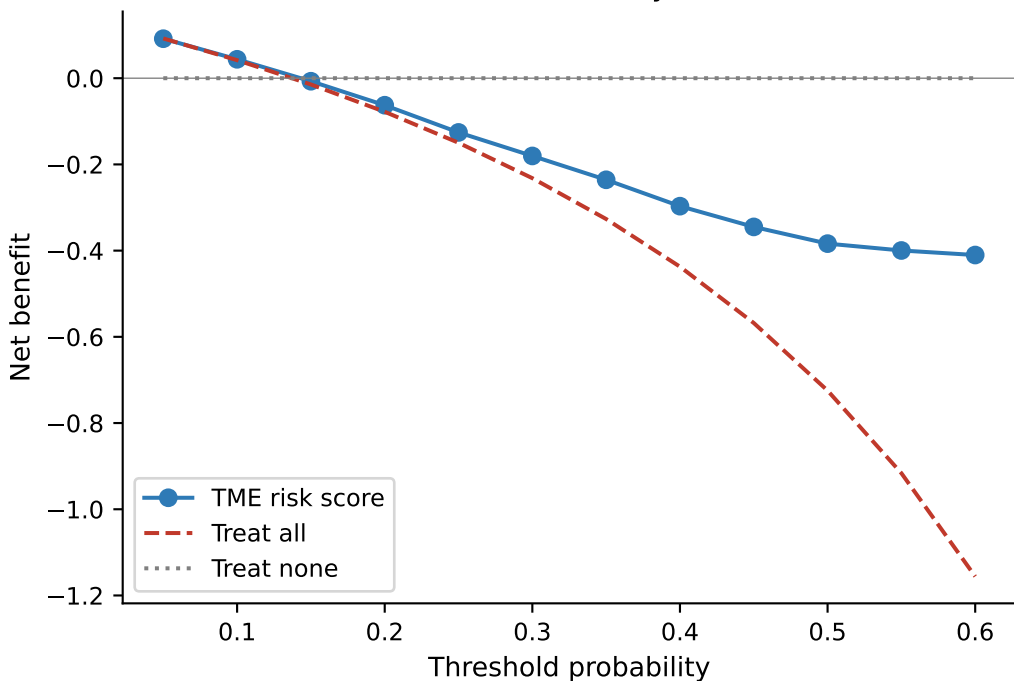
Decision Curve Analysis (OS)
