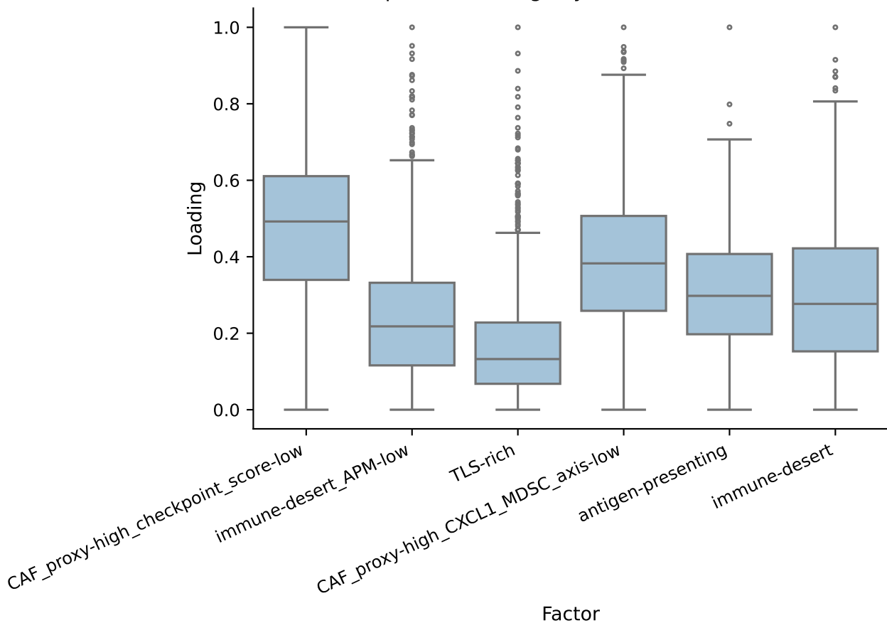
Per-patient loadings by factor (TCGA-BRCA)
