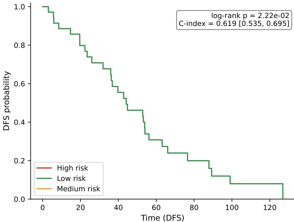
TME-risk-score tertile Kaplan-Meier (DFS)
