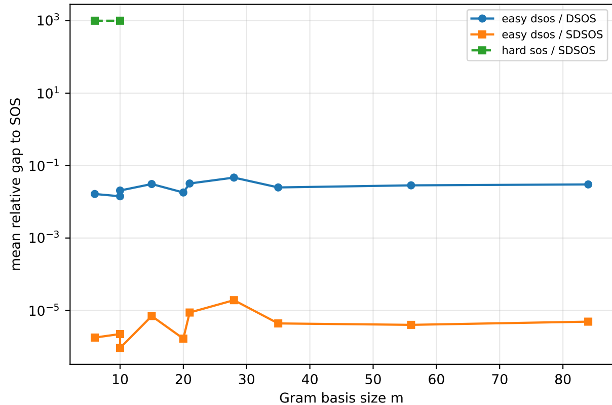
Benchmark I: gap to SOS versus Gram basis size
