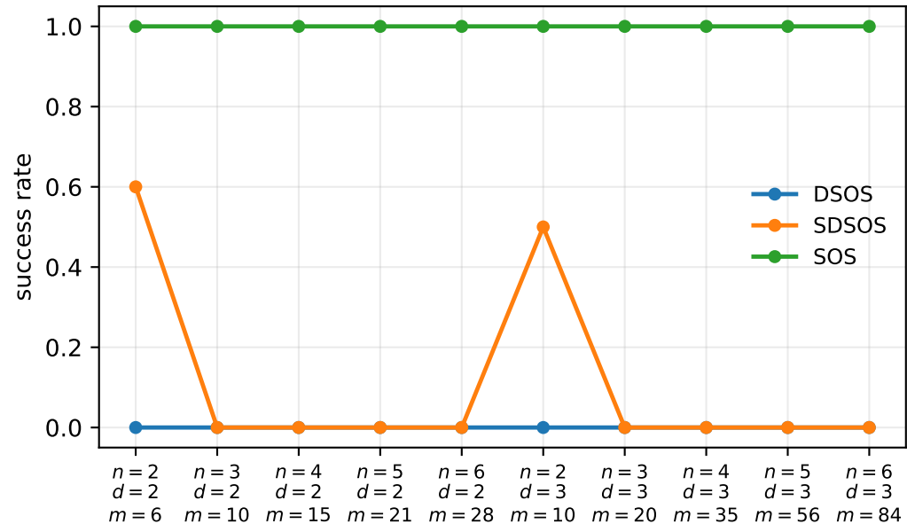
(b) Success on generic SOS instances
