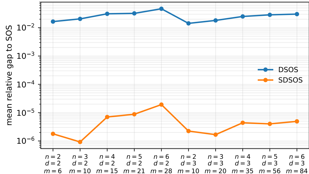
(a) Gap on DSOS-friendly instances
