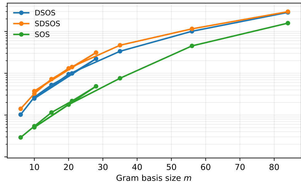
Random PSD Gram
