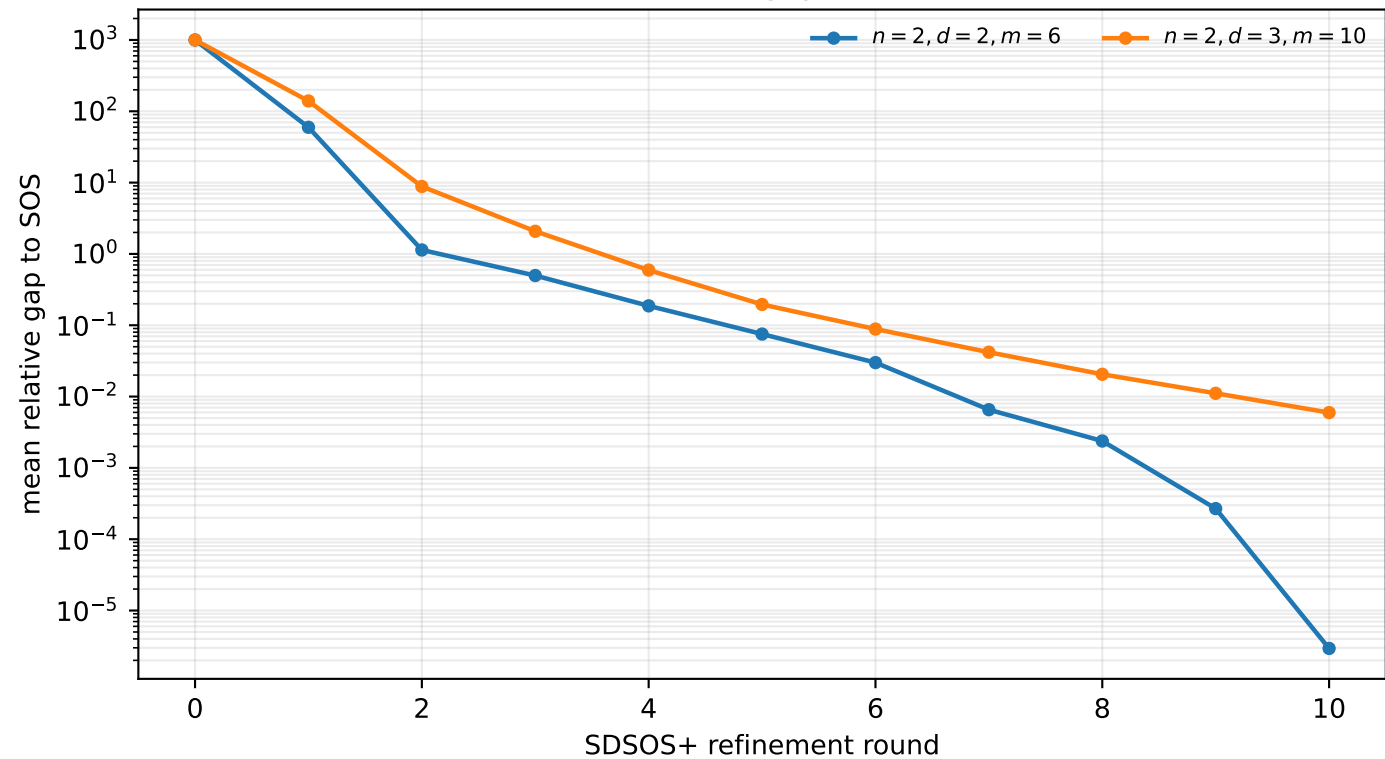
SDSOS+ closes the gap when initialized
