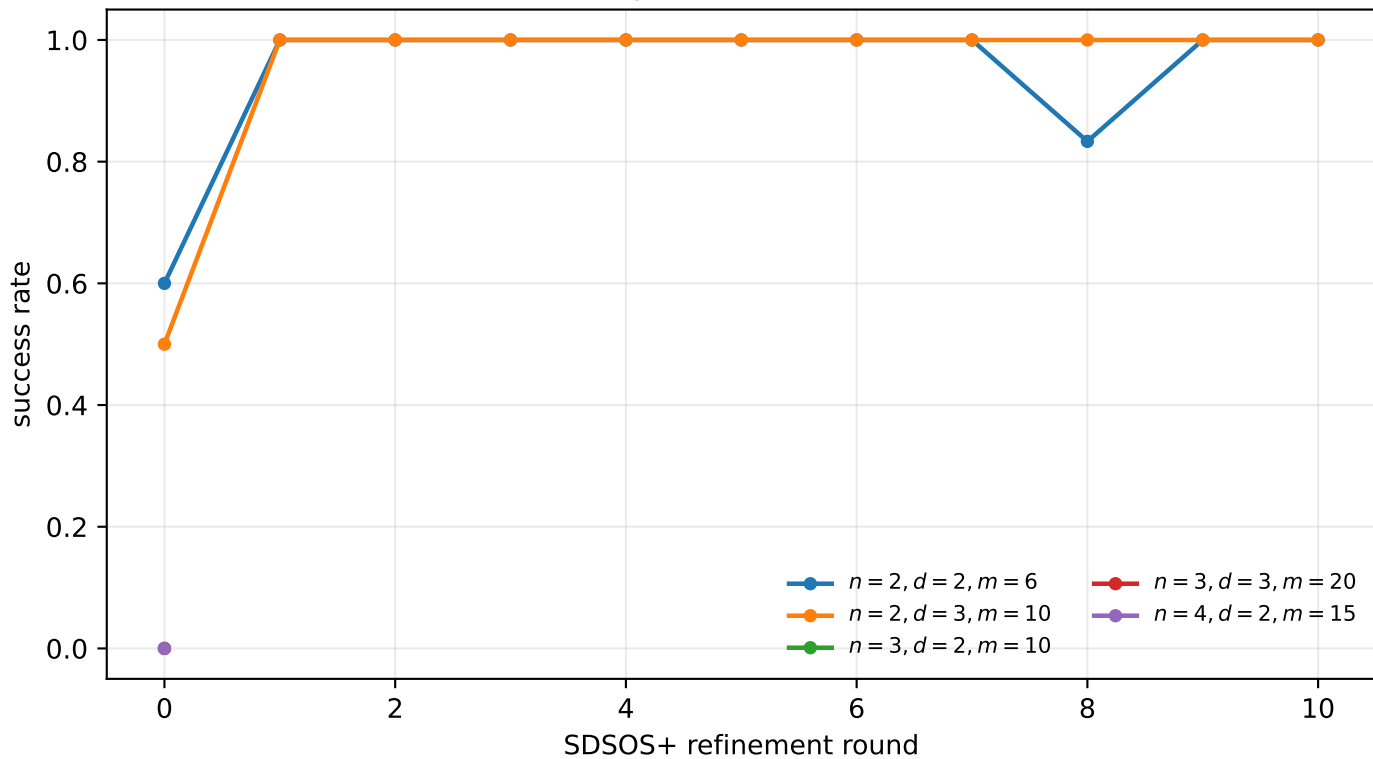
SDSOS+ feasibility over basis-refinement rounds
