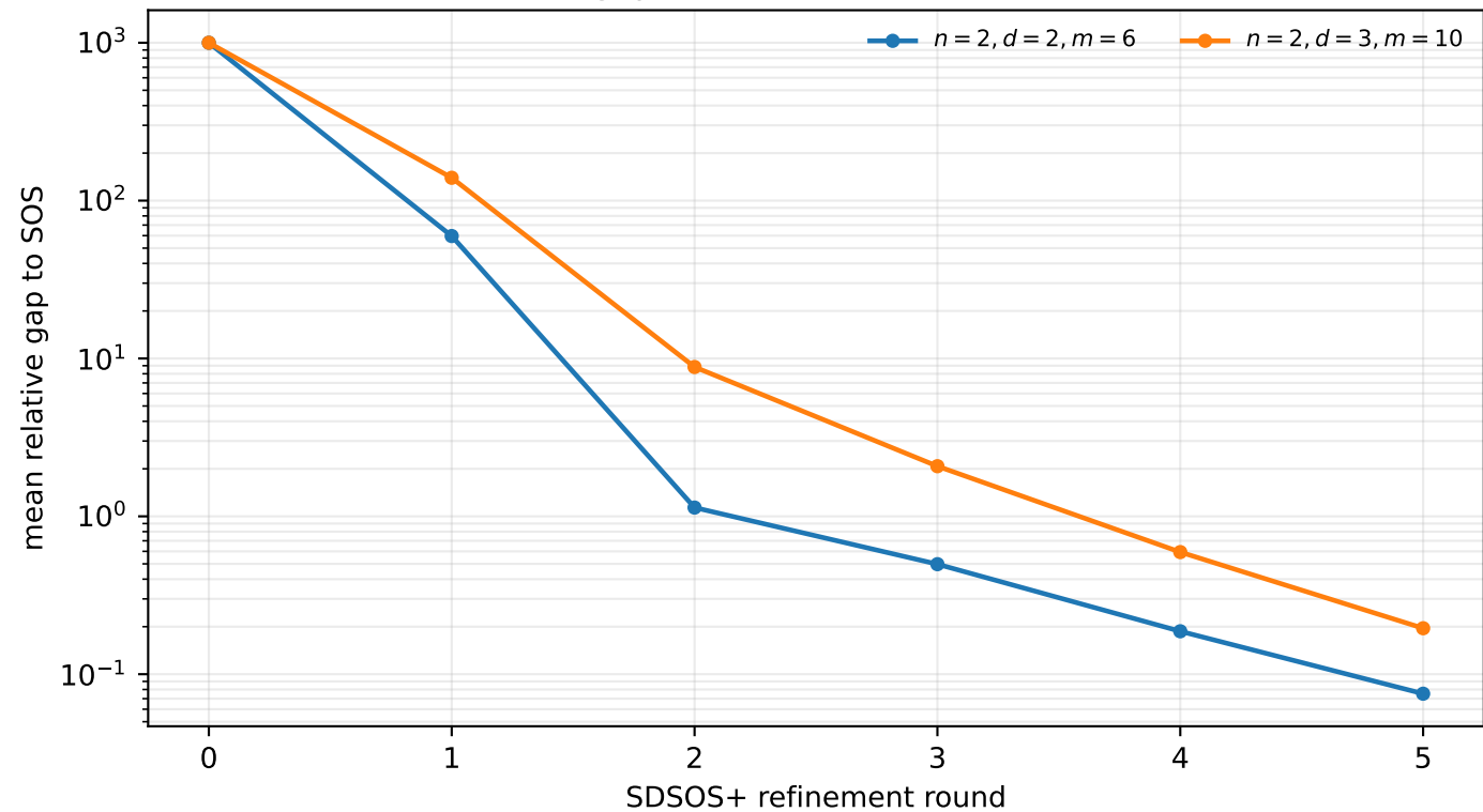
SDSOS+ gap to SOS over refinement rounds
