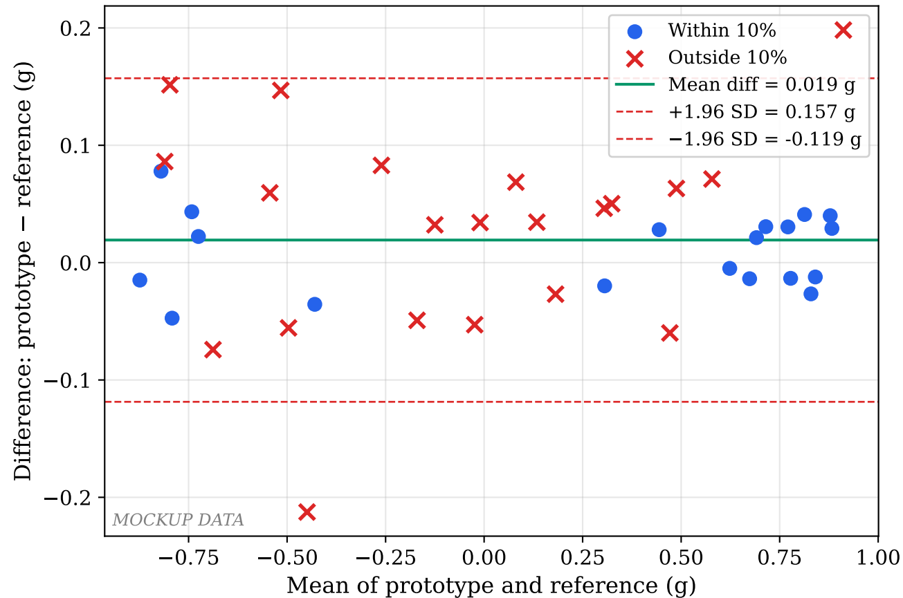
Bland-Altman: Accelerometer Pendulum Validation (n=40)
