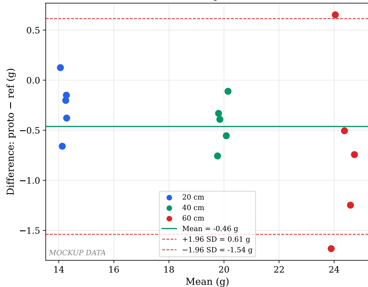
Bland-Altman: Drop-Test Validation
