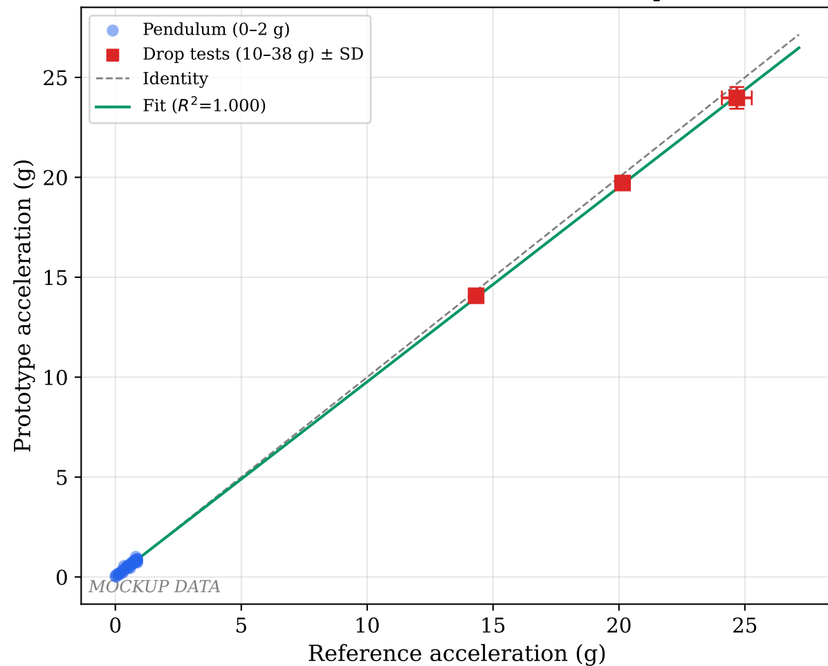
Extended Calibration: Pendulum + Drop Tests
