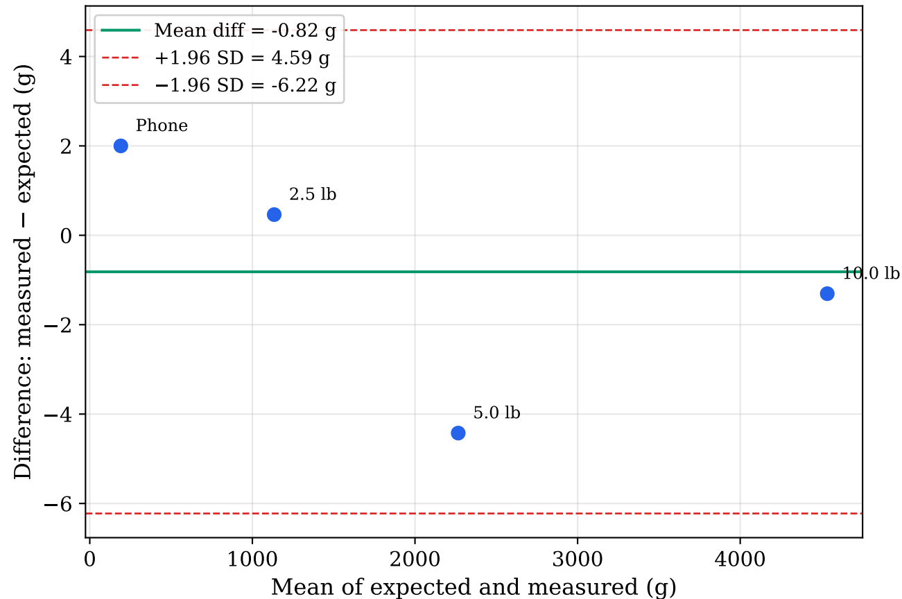
Bland-Altman Plot: Load-Cell Calibration
