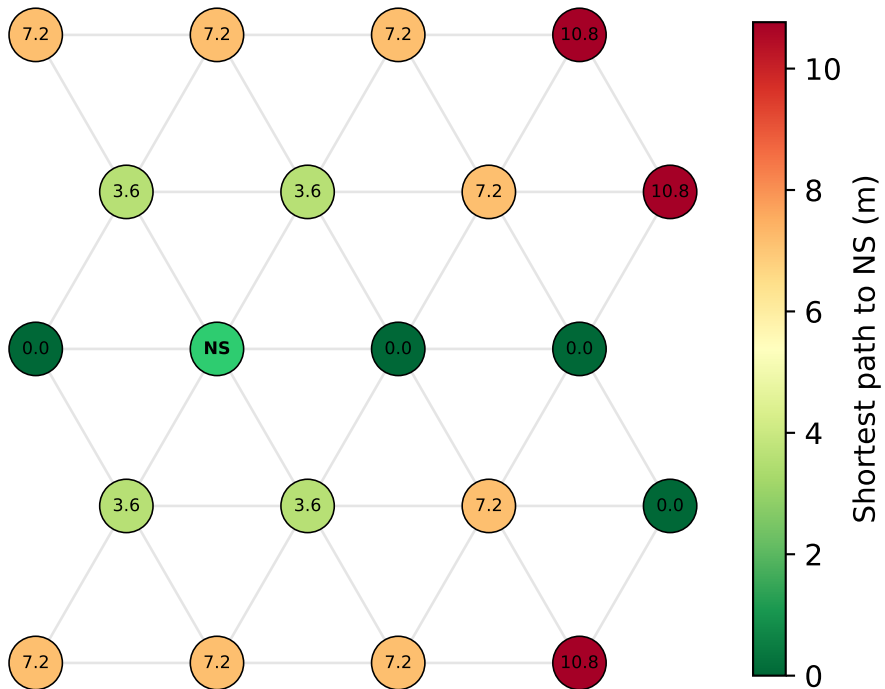
Hexagonal layout - distance heatmap (mean = 6.9 m)
