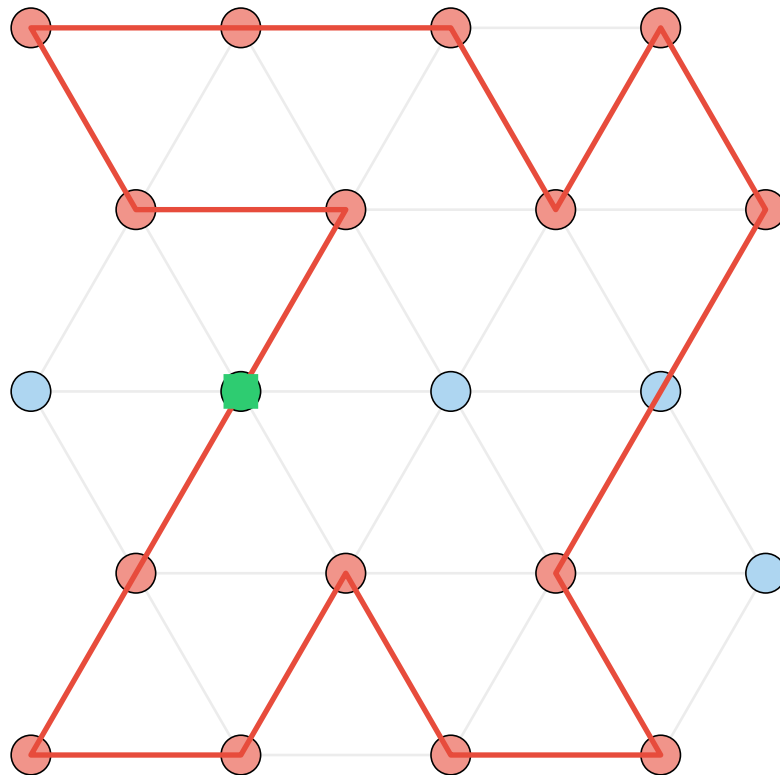
Hexagonal layout Optimal tour: 61.0 m
