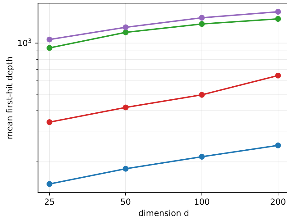
ZO fixed-configuration dimension sensitivity: absolute metrics
