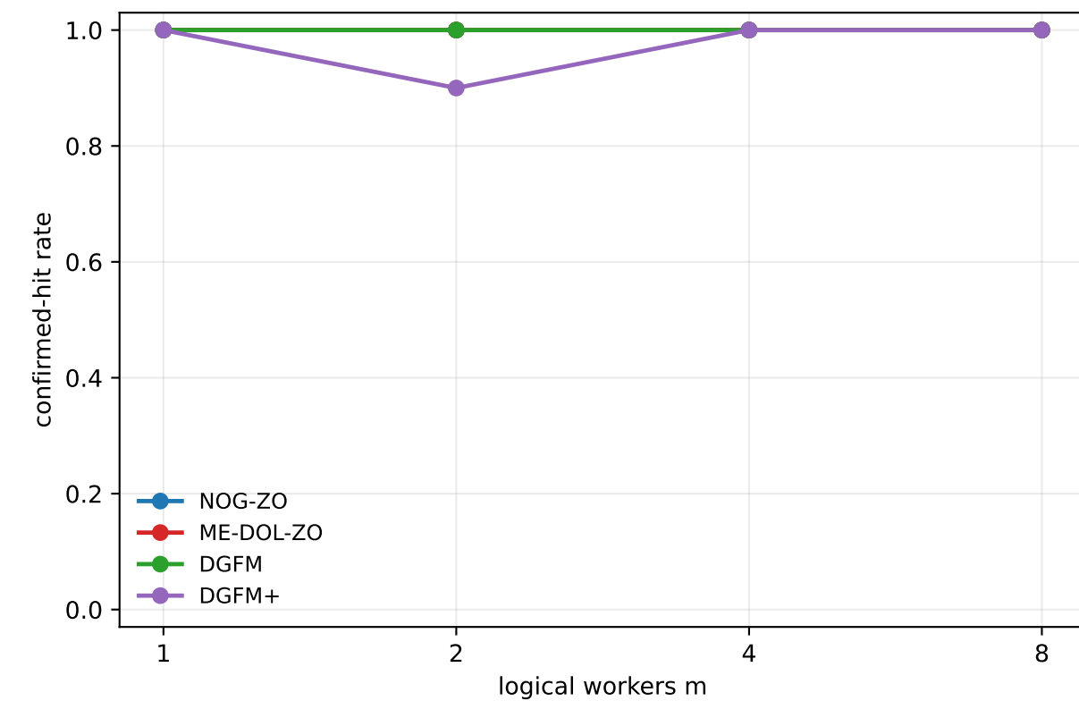
ZO fixed-configuration logical-worker sensitivity (epsilon=0.05)
