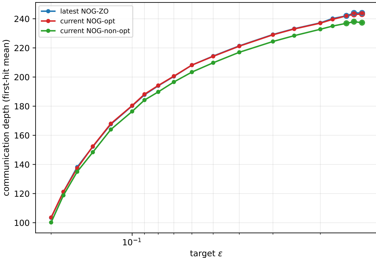
ZO NOG optimistic ablation: SyntheticMaxSinL1 Open markers: hit rate < 100%; zero-hit points omitted
