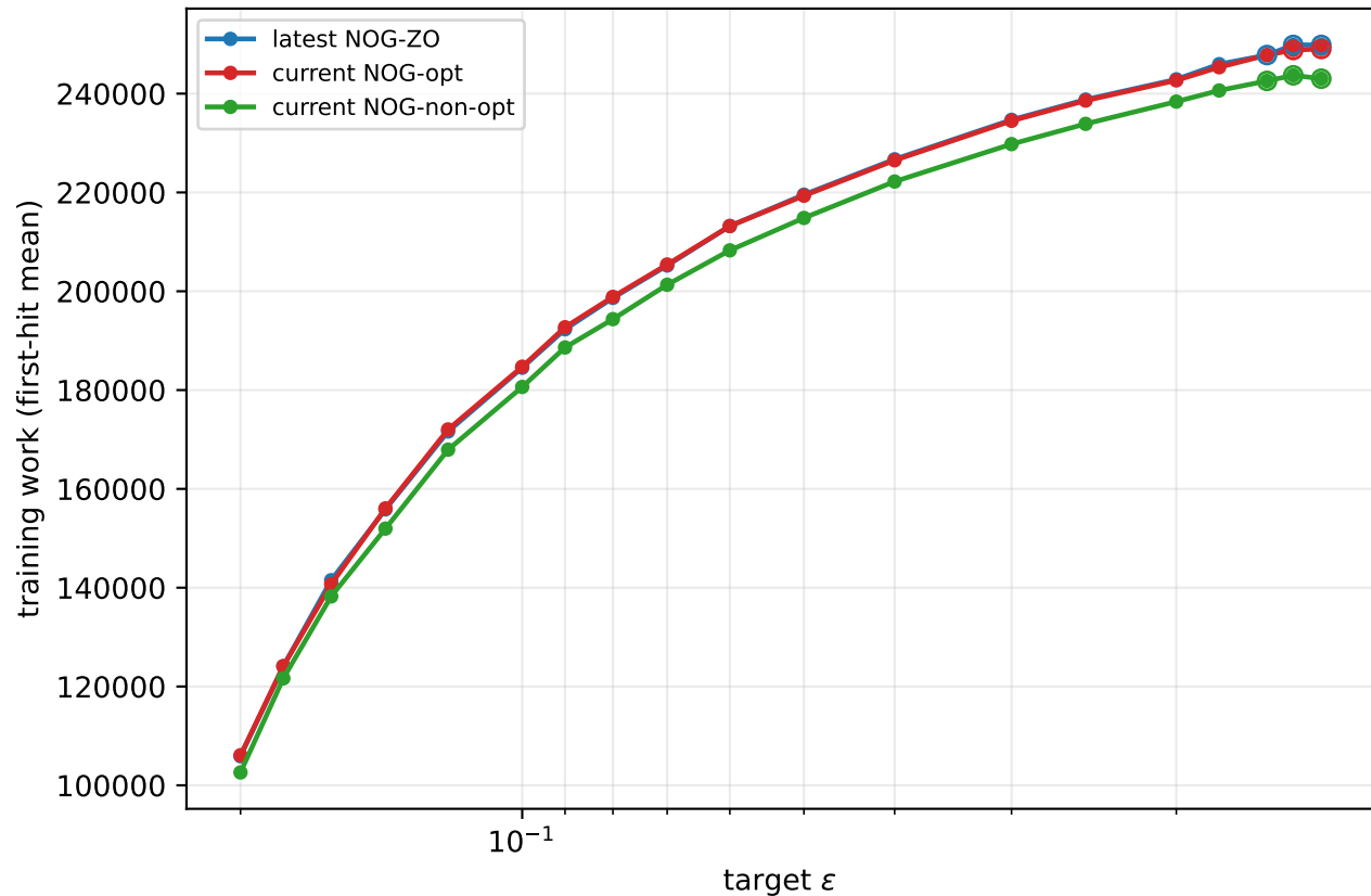
ZO NOG optimistic ablation: SyntheticMaxSinL1 Open markers: hit rate < 100%; zero-hit points omitted
