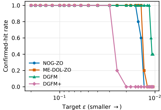
(a) Hit rate over five pilot seeds
