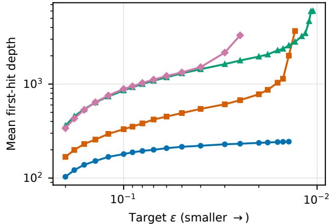
(b) Depth, conditional on hit
