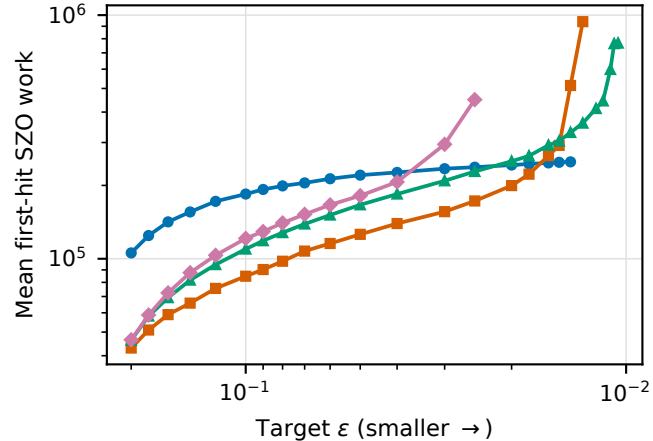
(c) Work, conditional on hit
